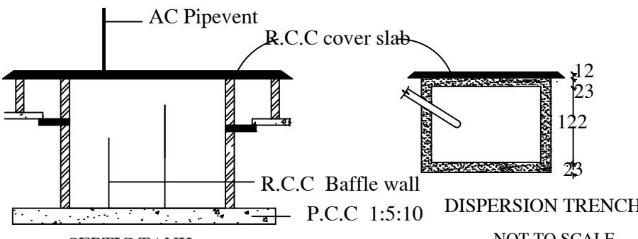
SEPTIC TANK
