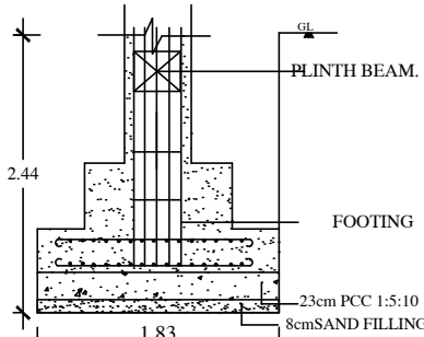
COLUMN FOUNDATION DETAILS NOT TO SCALE
