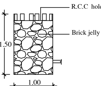
COLLECTING RAIN WATER PIT Not to Scale
