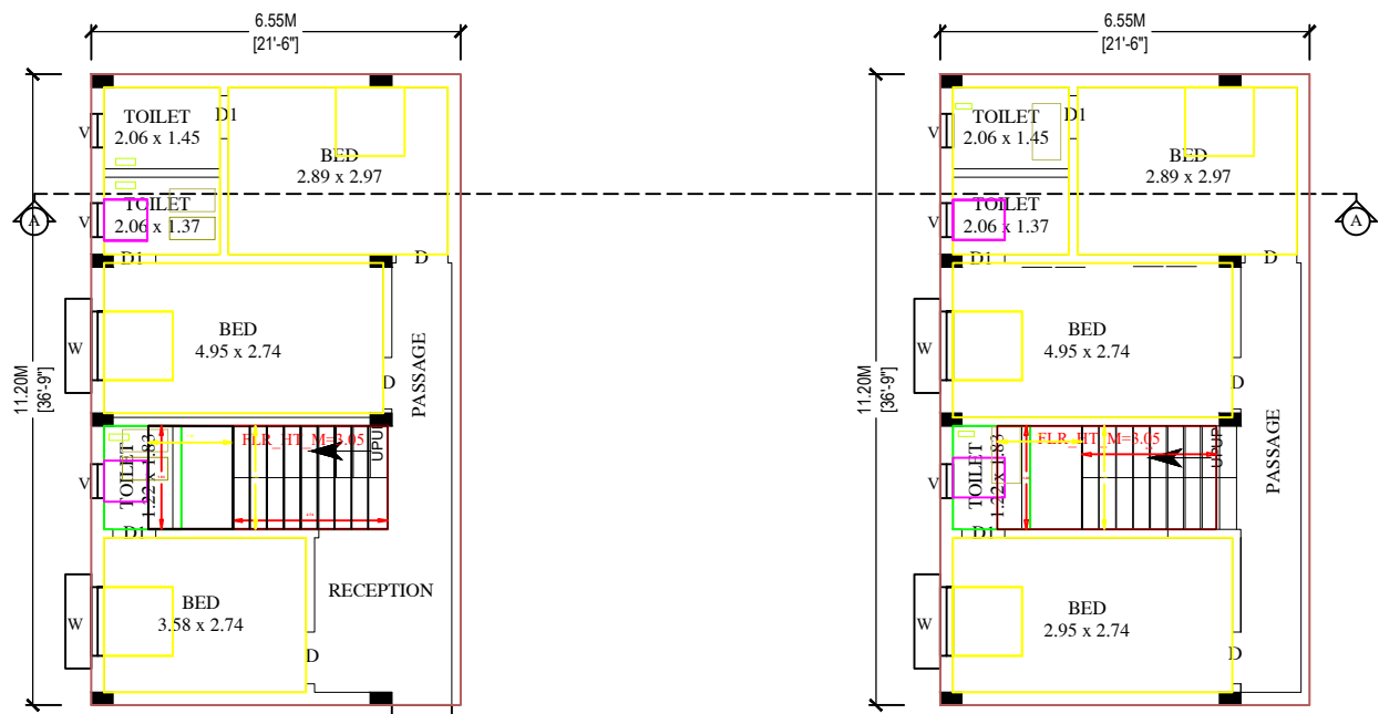
PRO.FIRST FLOOR PLAN
