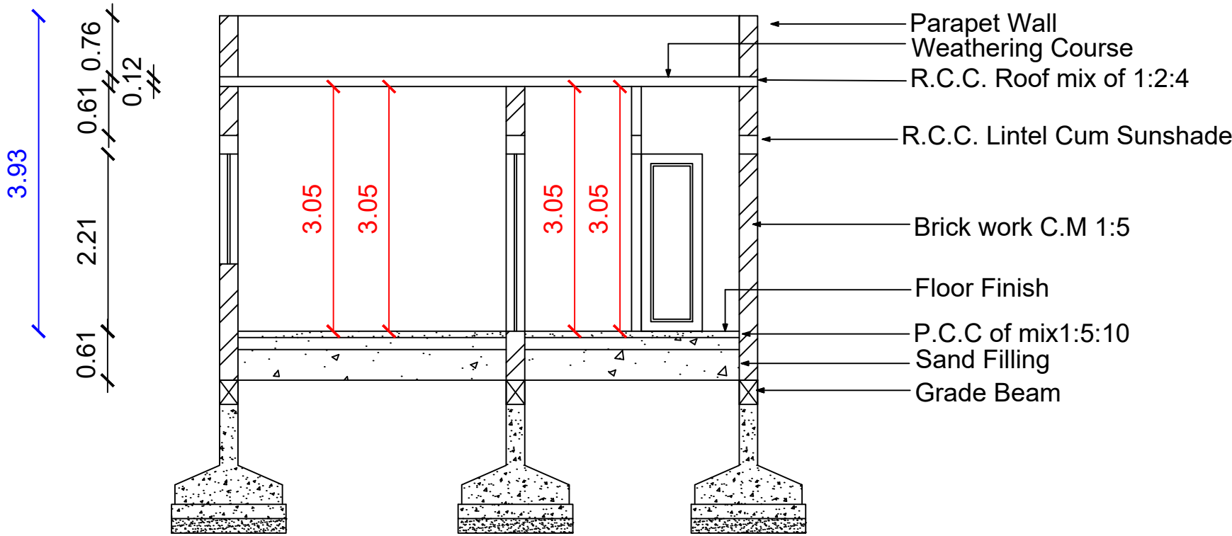
CROSS SECTION AB
