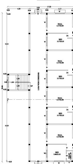
TYPICAL FLOOR PLAN BLOCK-2
