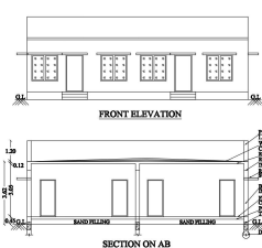
FRONT ELEVATION
