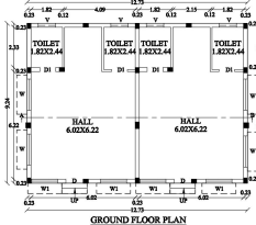
GROUND FLOOR PLAN BLOCK-2
