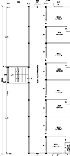
GROUND FLOOR PLAN BLOCK-2
