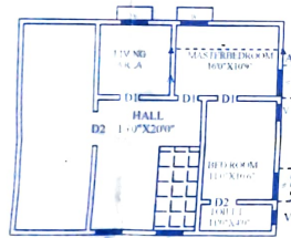
FIRST PLAN
