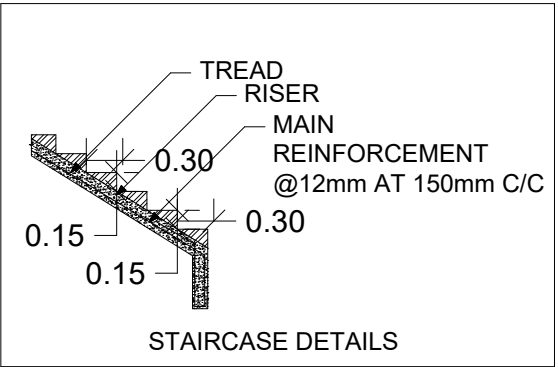
STAIRCASE DETAILS
