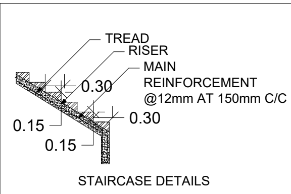
STAIRCASE DETAILS
