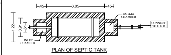
DETAILS OF SEPTIC TANK ( N.T.S.)
