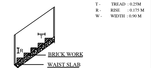
STAIRCASE & ENTRANCE STEPS
