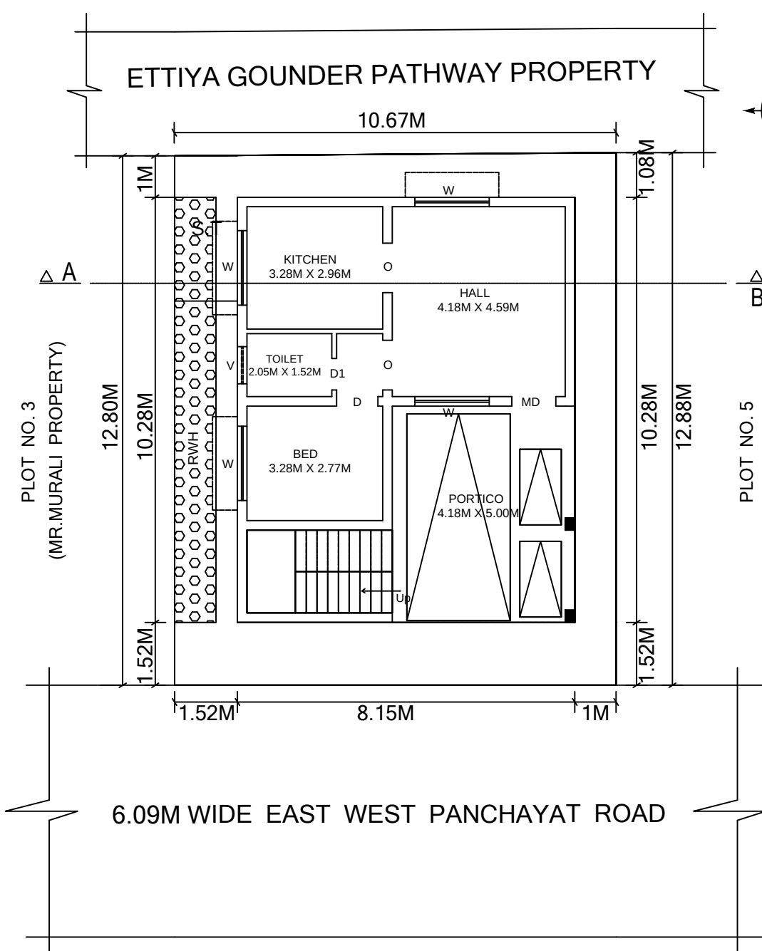
SITE PLAN CUM GROUND FLOOR PLAN
