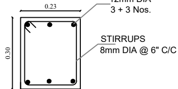
ROOF BEAM SECTION
