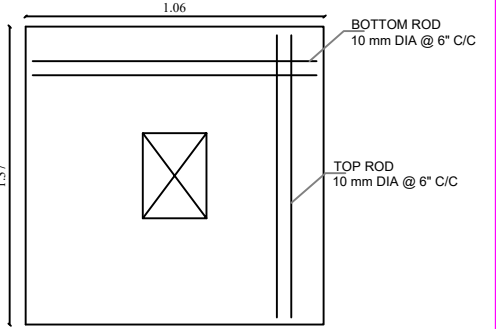
FOOTING PLAN
