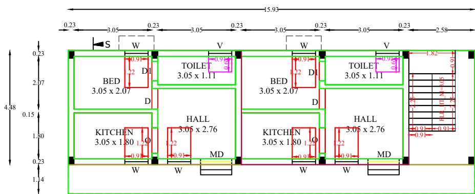
PROPOSED GROUND FLOOR PLAN
