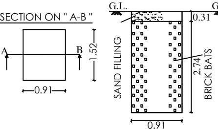
DETAILED PLAN OF RAINWATER PERCOLATION AND COLLECTION PIT
