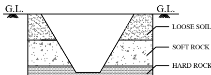
TRIAL PIT
