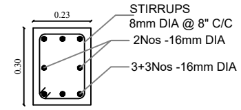
COLUMN PLAN
