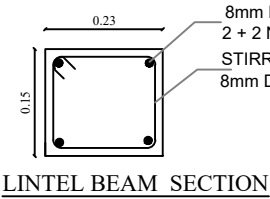
LINTEL BEAM SECTION
