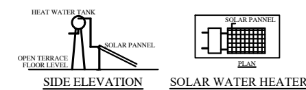
SIDE ELEVATION
