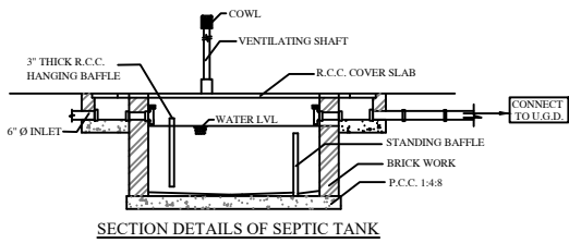
SECTION DETAILS OF SEPTIC TANK
