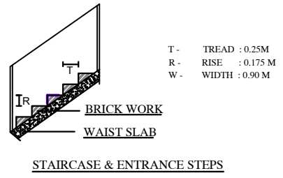
STAIRCASE & ENTRANCE STEPS
