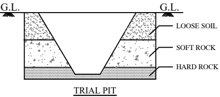
TRIAL PIT
