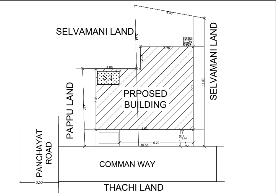
SITE PLAN / LOCATION PLAN
