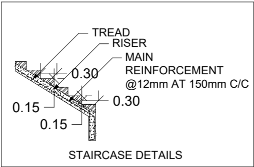
STAIRCASE DETAILS
