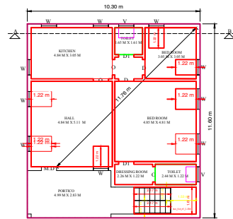
PLAN [NORTH FACING]
