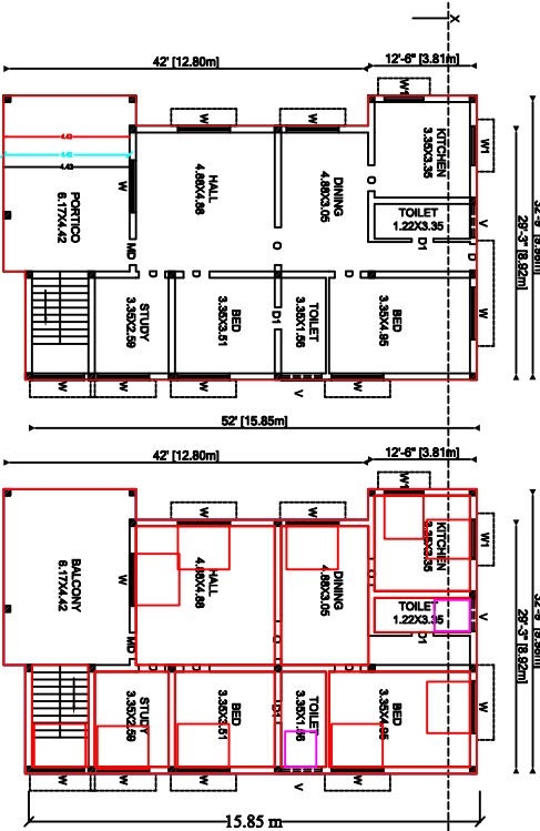
GROUND FLOOR PLAN. [EXISTING]
