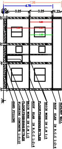
SECTION ON-X-Y
