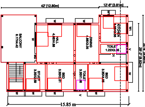
FIRST FLOOR PLAN. [PROPOSED]
