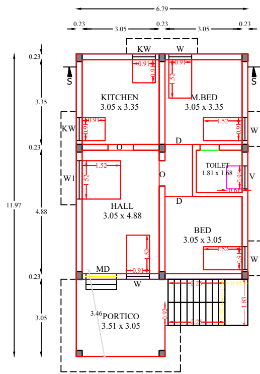
PROPOSED GROUND FLOOR PLAN PLAN : 1:100
