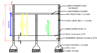
SECTION"AB"
