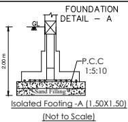
Isolated Footing -A (1.50X1.50) (Not to Scale)
