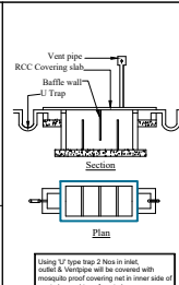
Joineries
