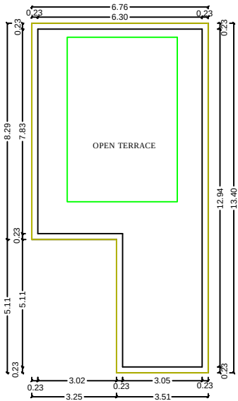
PROPOSED TERRACE FLOOR PLAN
