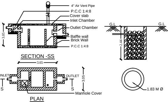
SEPTIC TANK & SOAK PIT DETAILS
