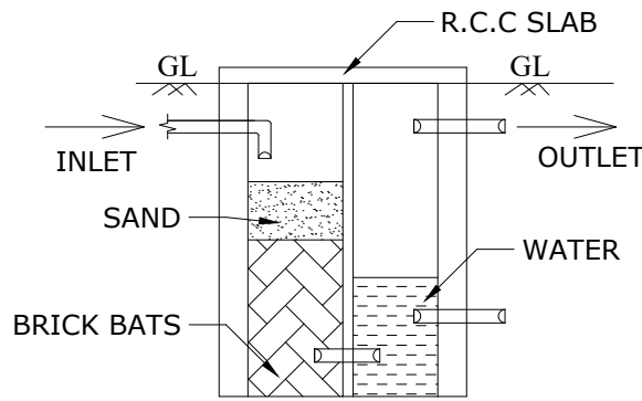
RAIN WATER COLLECTION PIT
