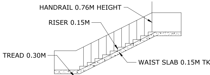
STAIRCASE DETAILS
