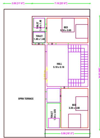
FIRST FLOOR PLAN WEST FACING
