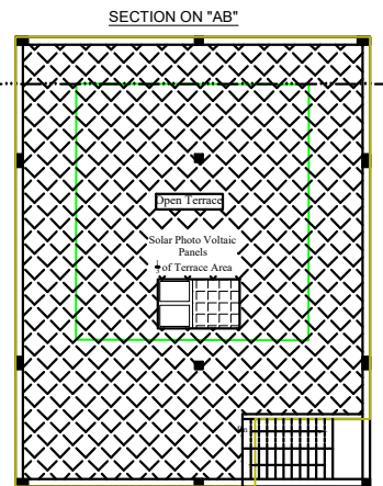
ROOF FLOOR PLAN SCALE:1:100
