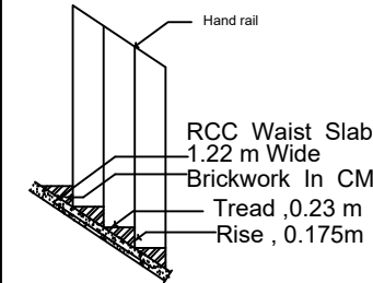
STAIRCASE DETAILS SECTION
