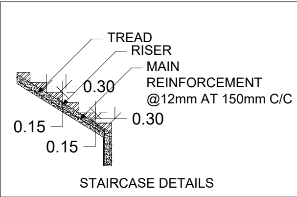
STAIRCASE DETAILS
