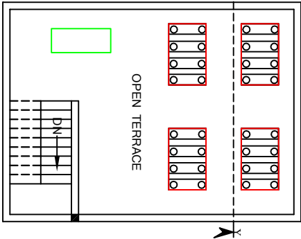
Terrace Floor Plan. (Scale - 1:100)
