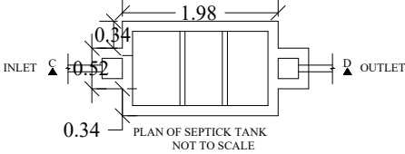
PLAN OF SEPTICK TANK NOT TO SCALE
