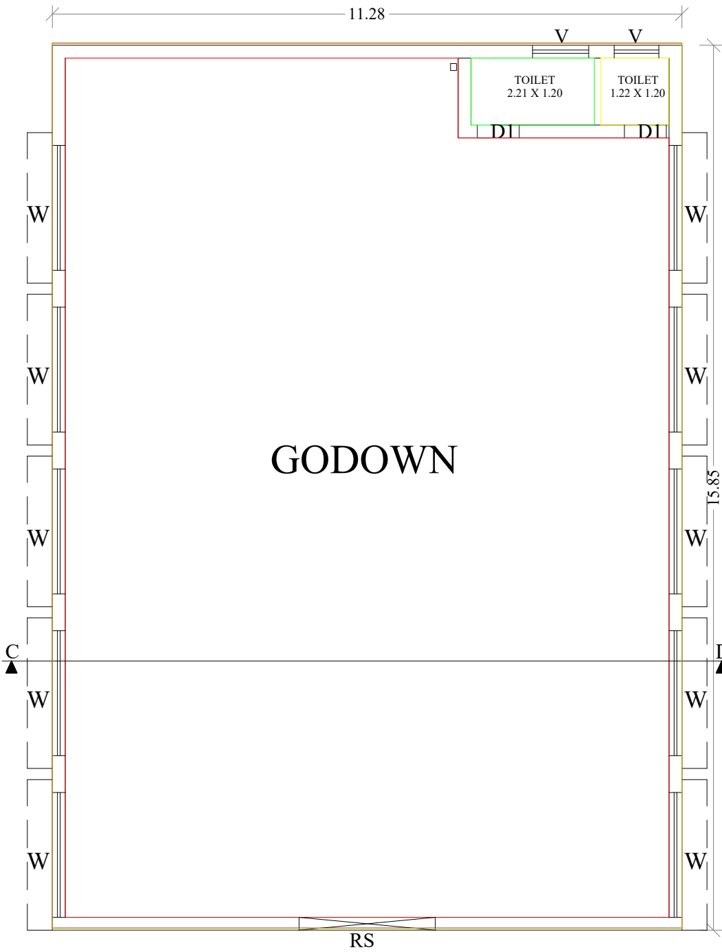
GROUND FLOORPLAN
