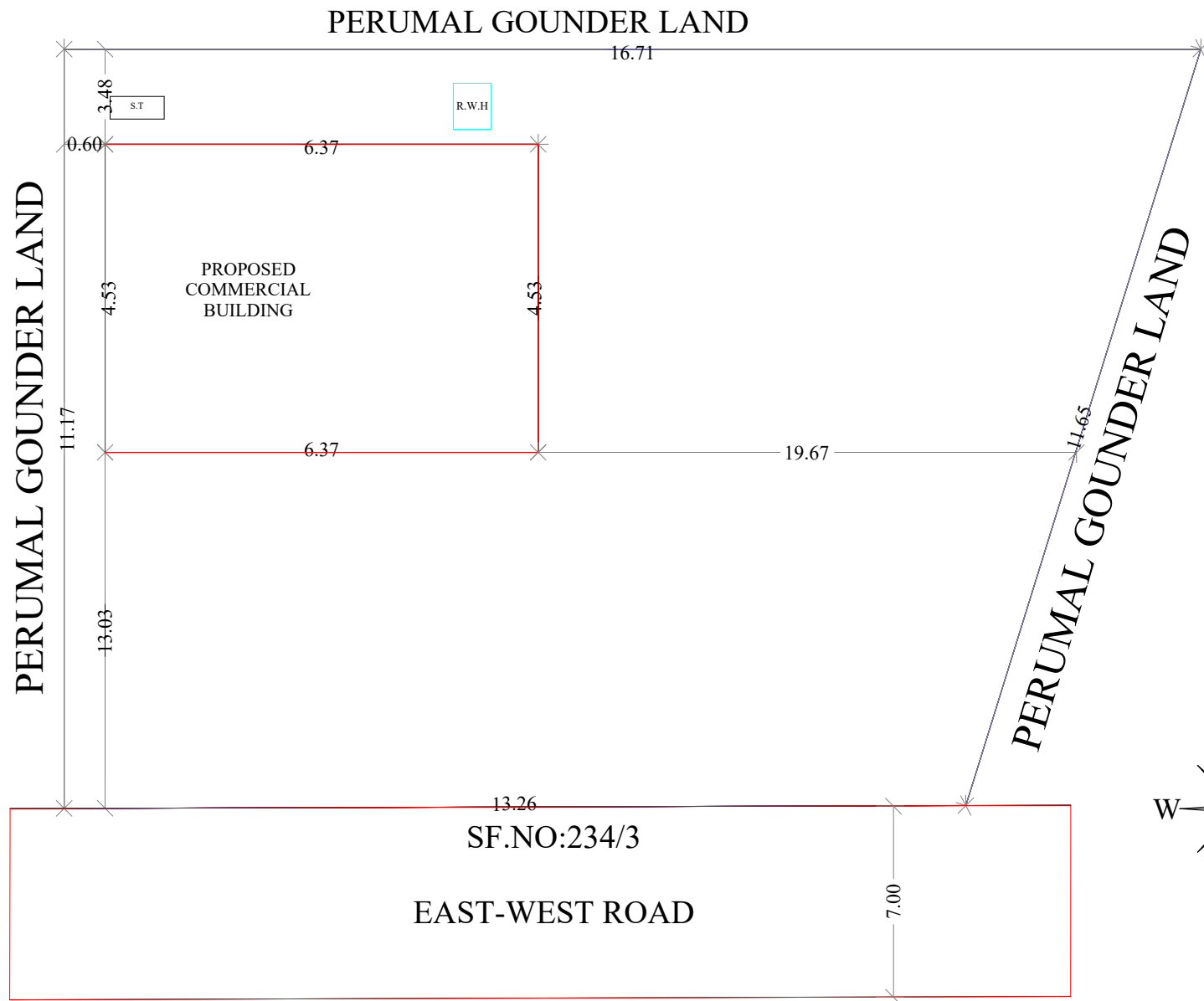
SITE PLAN NOT TO SCALE
