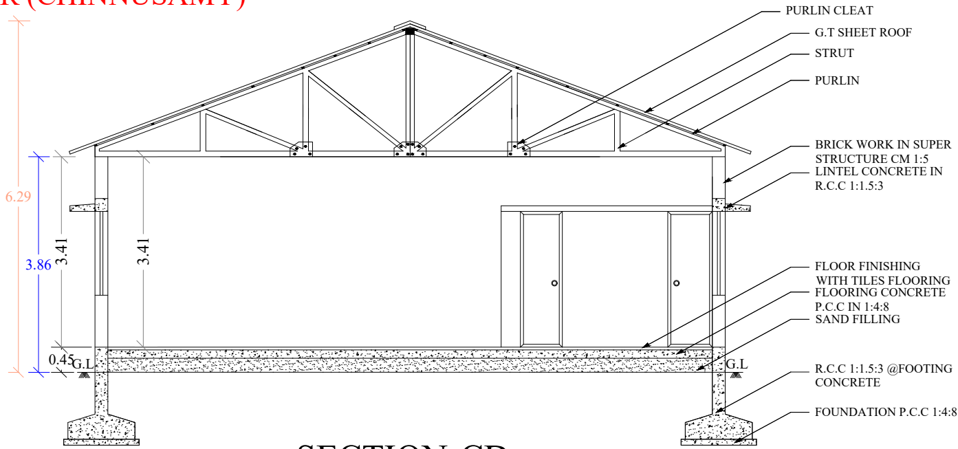
SECTION-CD
