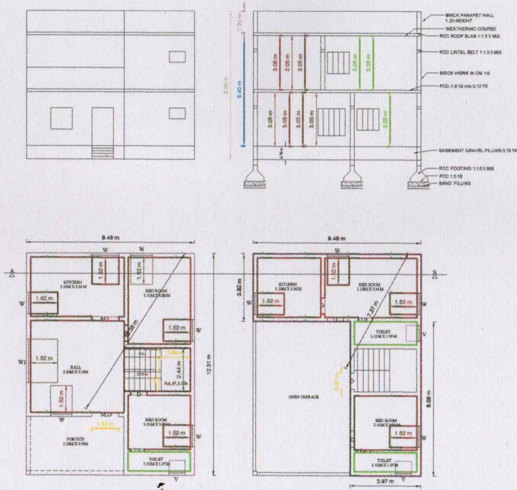
G.F PLAN [NORTH FACING]
