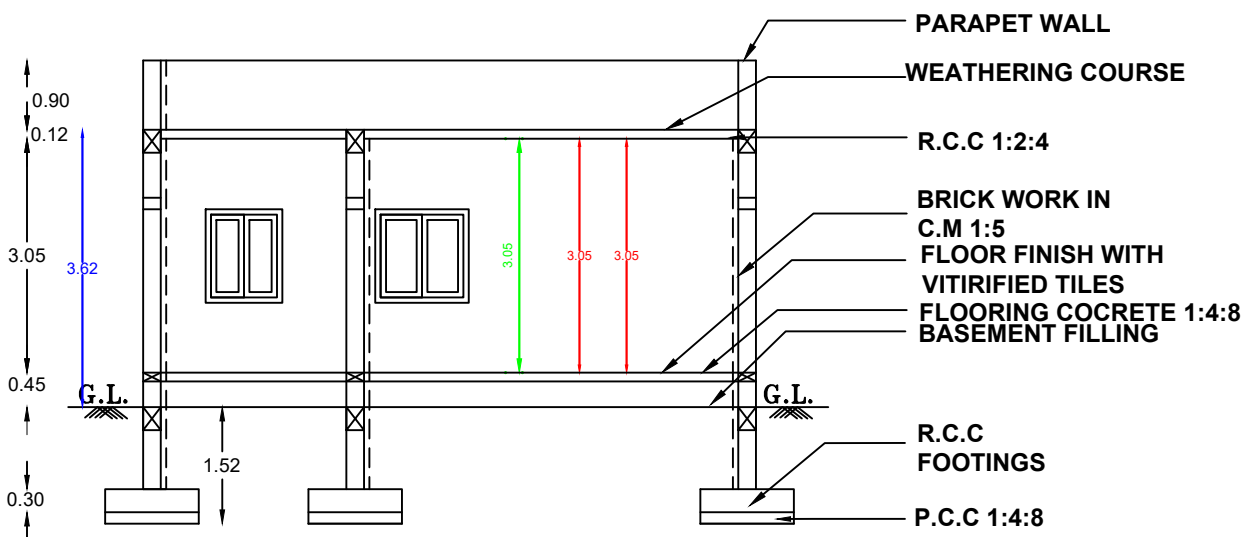
SECTION ON "S S"
