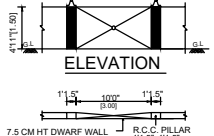
COMPOUND WALL PLAN
