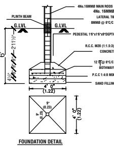
FOUNDATION DETAIL
