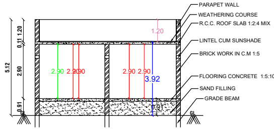
SECTION-AB
