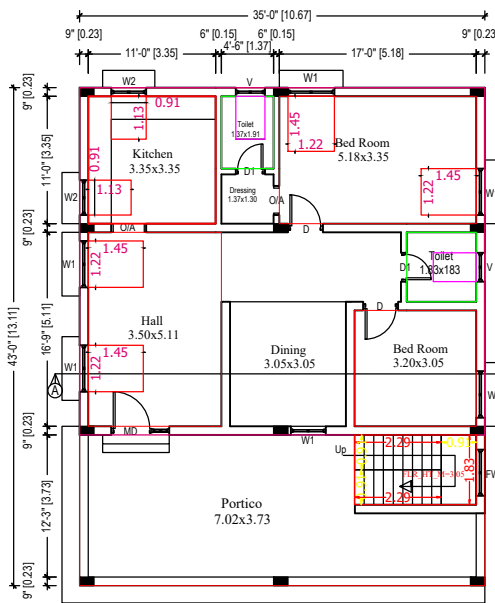
EXIGROUND FLOOR PLAN
