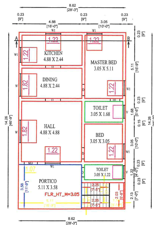
PLAN Scale (1:100)
