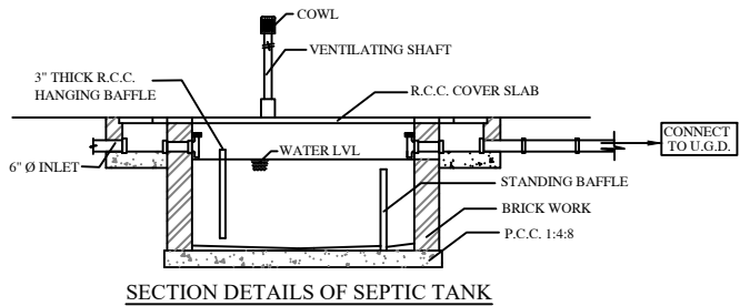
SECTION DETAILS OF SEPTIC TANK
