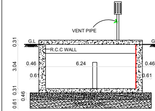
SECTION ON B-B
