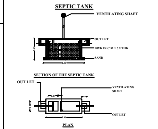
SEPTIC TANK
