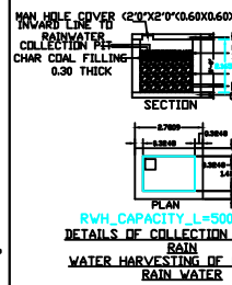
SECTION ON AA
