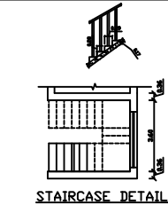
STAIRCASE DETAIL
