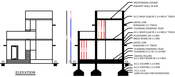
SECTION A TO B
