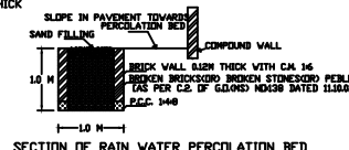
SECTION OF RAIN WATER PERCOLATION BED
