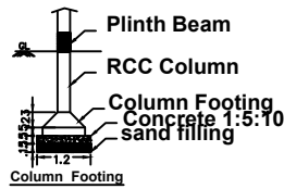
Foundation Detail
