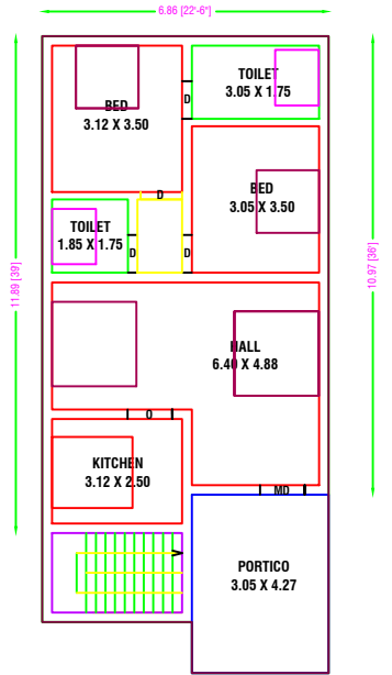
PRO. GROUND FLOOR
