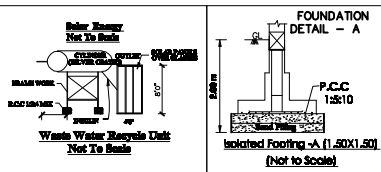
FOUNDATION DETAIL - A
