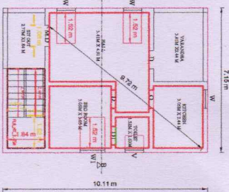
PLAN [WEST FACING]
