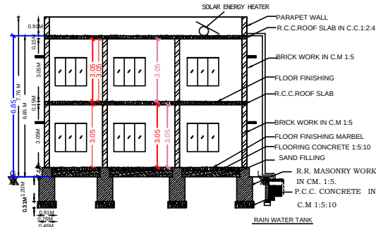
SECTION - XX
