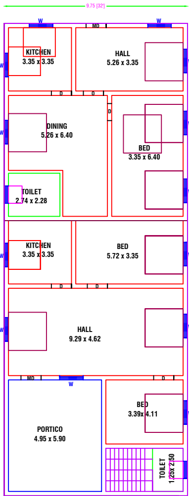
EX. GROUND FLOOR PLAN [ NORTH FACING ]
