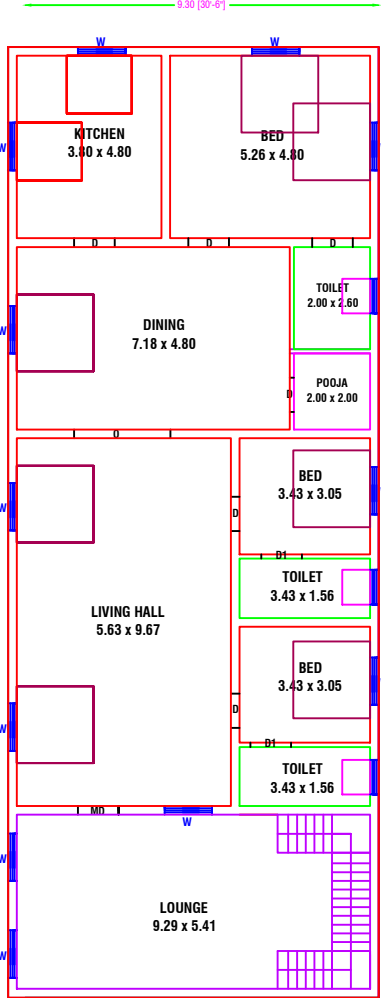
PRO FIRST FLOOR PLAN [ NORTH FACING ]
