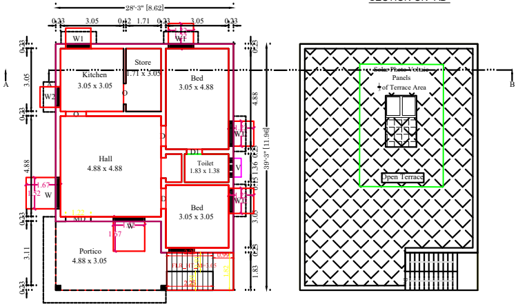
ROOF FLOOR PLAN SCALE:1:100
