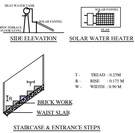
STAIRCASE & ENTRANCE STEPS
