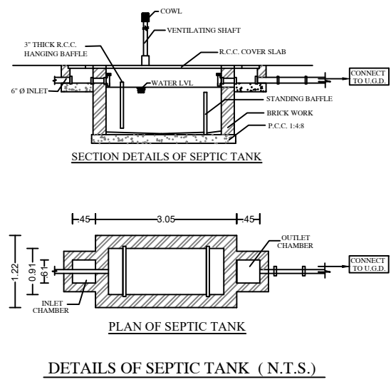
DETAILS OF SEPTIC TANK ( N.T.S. )
