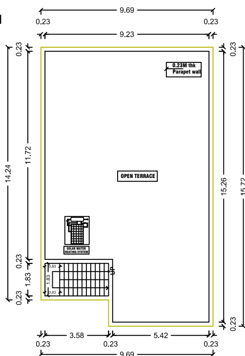
PRO.TERRACE FLOOR PLAN
