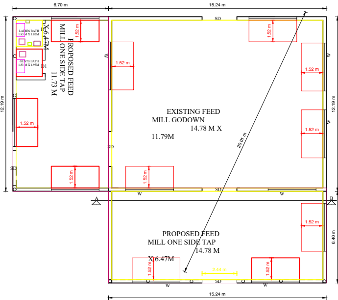
FEED MILL - GODOWN
