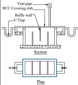
Section
