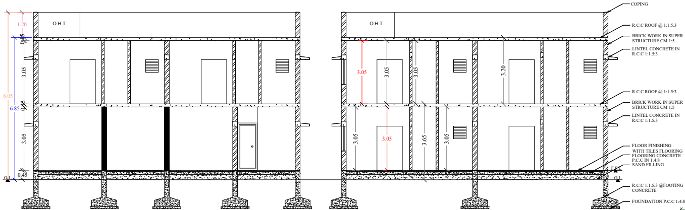
SECTION-AB
