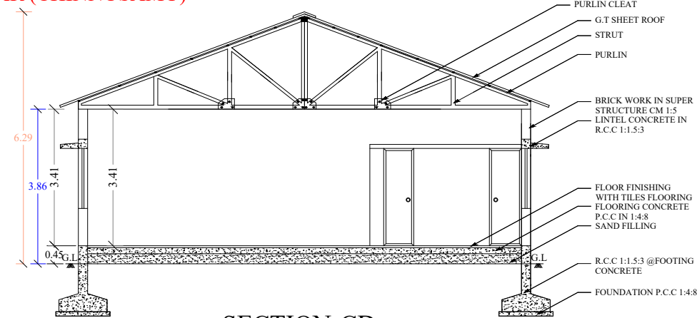
SECTION-CD
