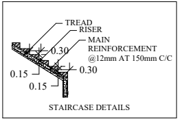
STAIRCASE DETAILS
