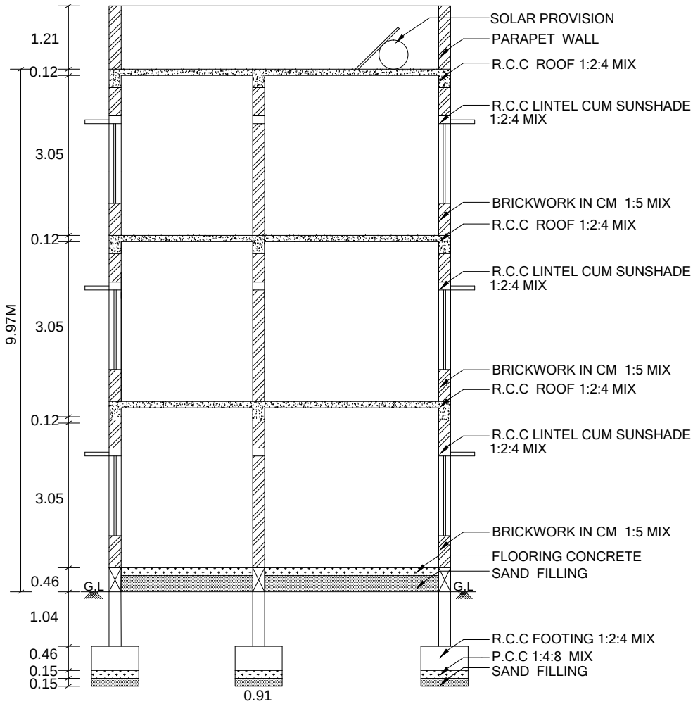
SECTION ON 'ABCD'
