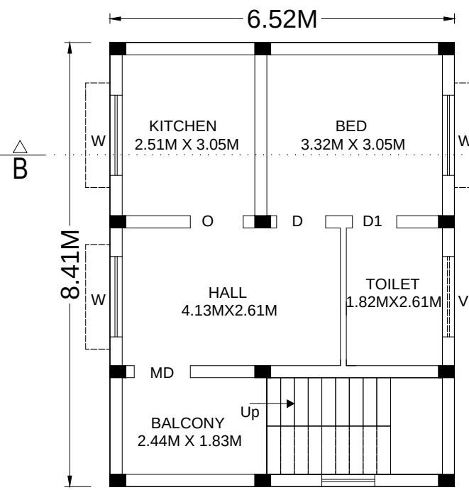
TYPICAL FLOOR PLAN (FIRST & SECOND FLOOR PLAN)
