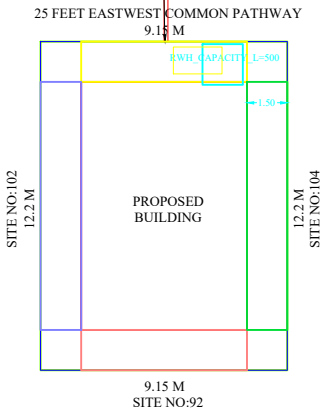
SITE PLAN
