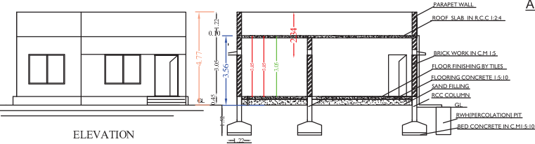
SECTION ON-XY
